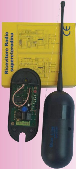
Radio Receiver Rolling Code Model: RX Mini Frequency: 433,92 Mhz Superheterodyne hybrid
