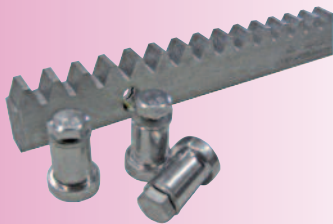
Galvanized iron rack 12x30x1000 Mod. 4 with solder connections included (slotted) Model: CR-FZ
