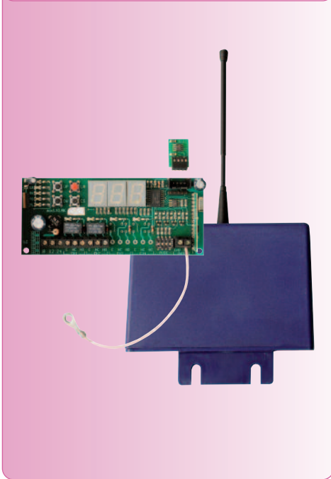
Radio Receiver Rolling Code with viewer and memory Model: RX Klak Frequency: 433,92 Mhz Superheterodyne hybrid
