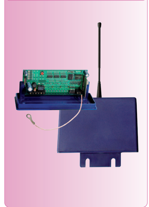
Radio Receiver Self-learning Model: RX Big Frequency: 433,92 Mhz Superheterodyne hybrid
