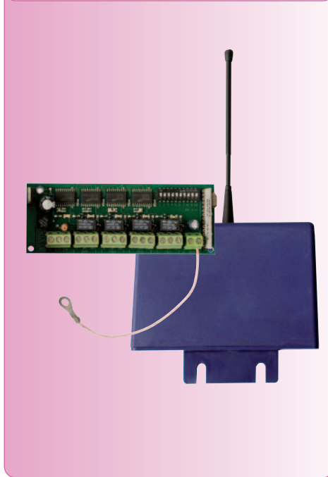
Radio Receiver Dip Switch Model: RX Big Frequency: 433,92 Mhz Superheterodyne hybrid
