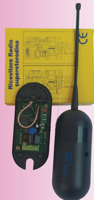
Radio Receiver Self-learning Model: RX Mini Frequency: 433,92 Mhz Superheterodyne hybrid
